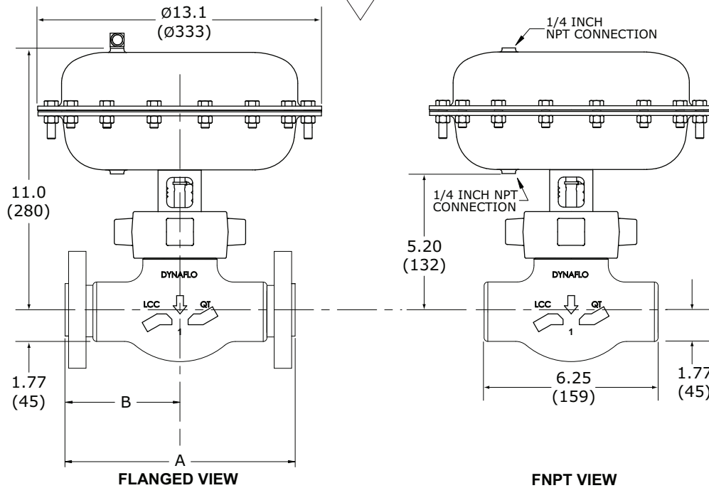
Figure 5 DF270 2 inch Control Valve Dimensions inch (mm)
