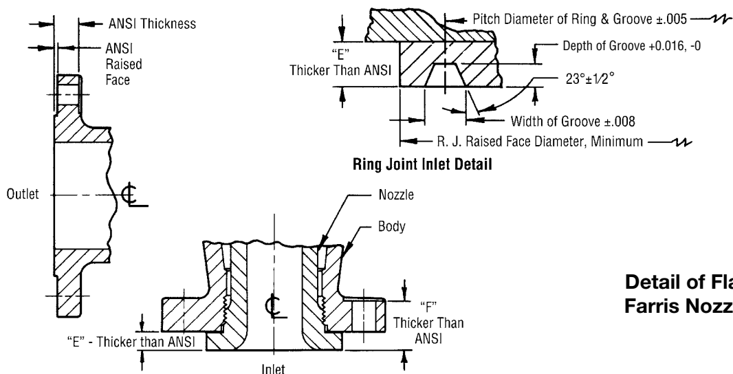
Full Nozzle Inlet Facings (Reference ANSI B16.5)
