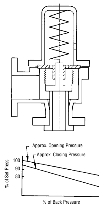
Unbalanced Bellows
