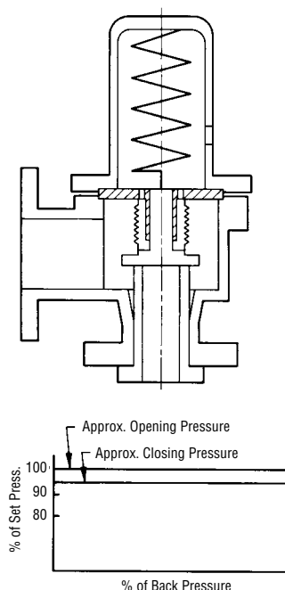
Balanced Farris Bellows
